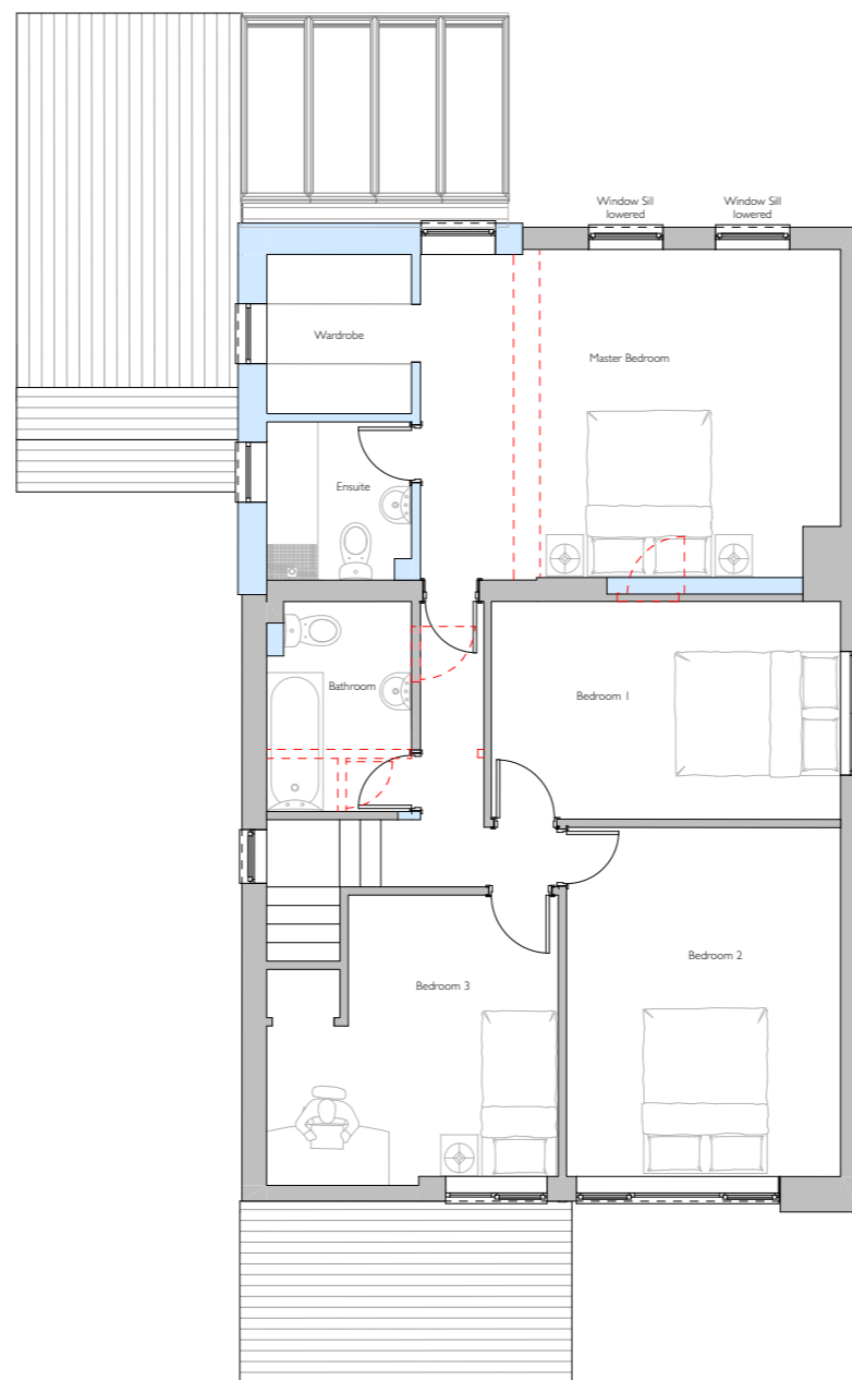
First Floor
