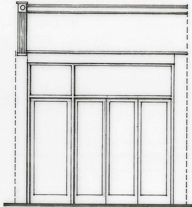
FRONT ELEV. 1:50
