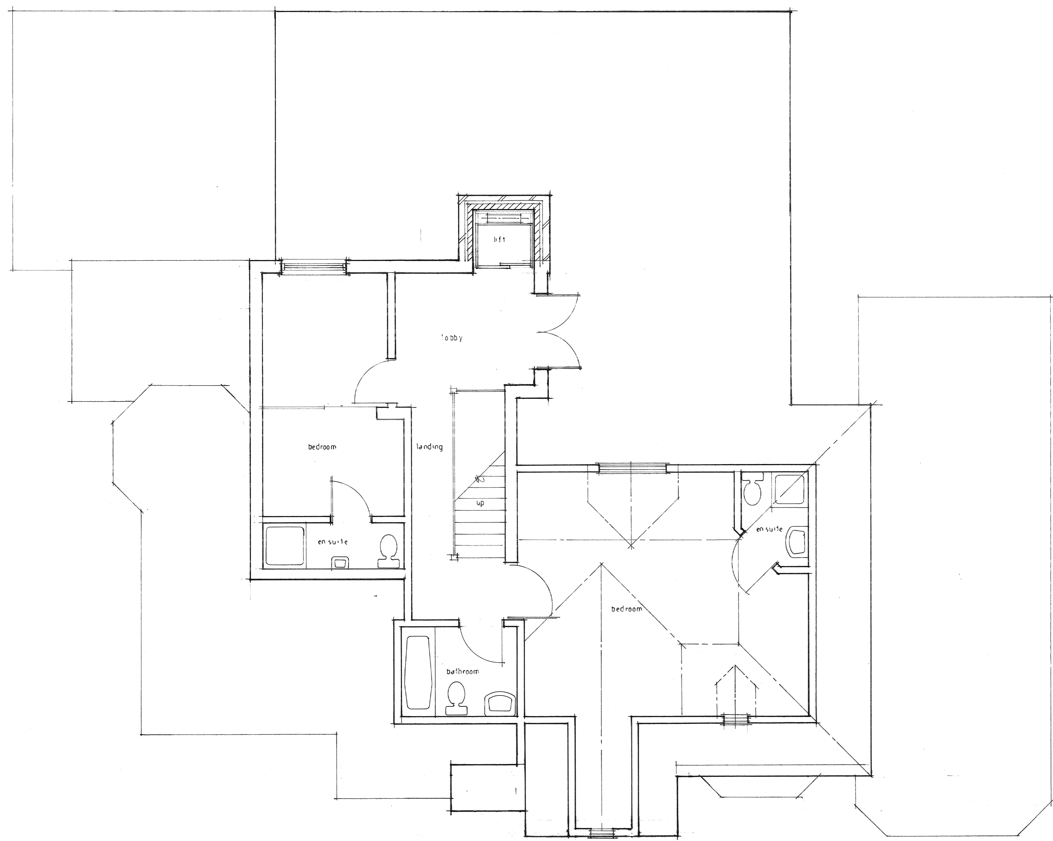
proposed attic plan scale 1/50
