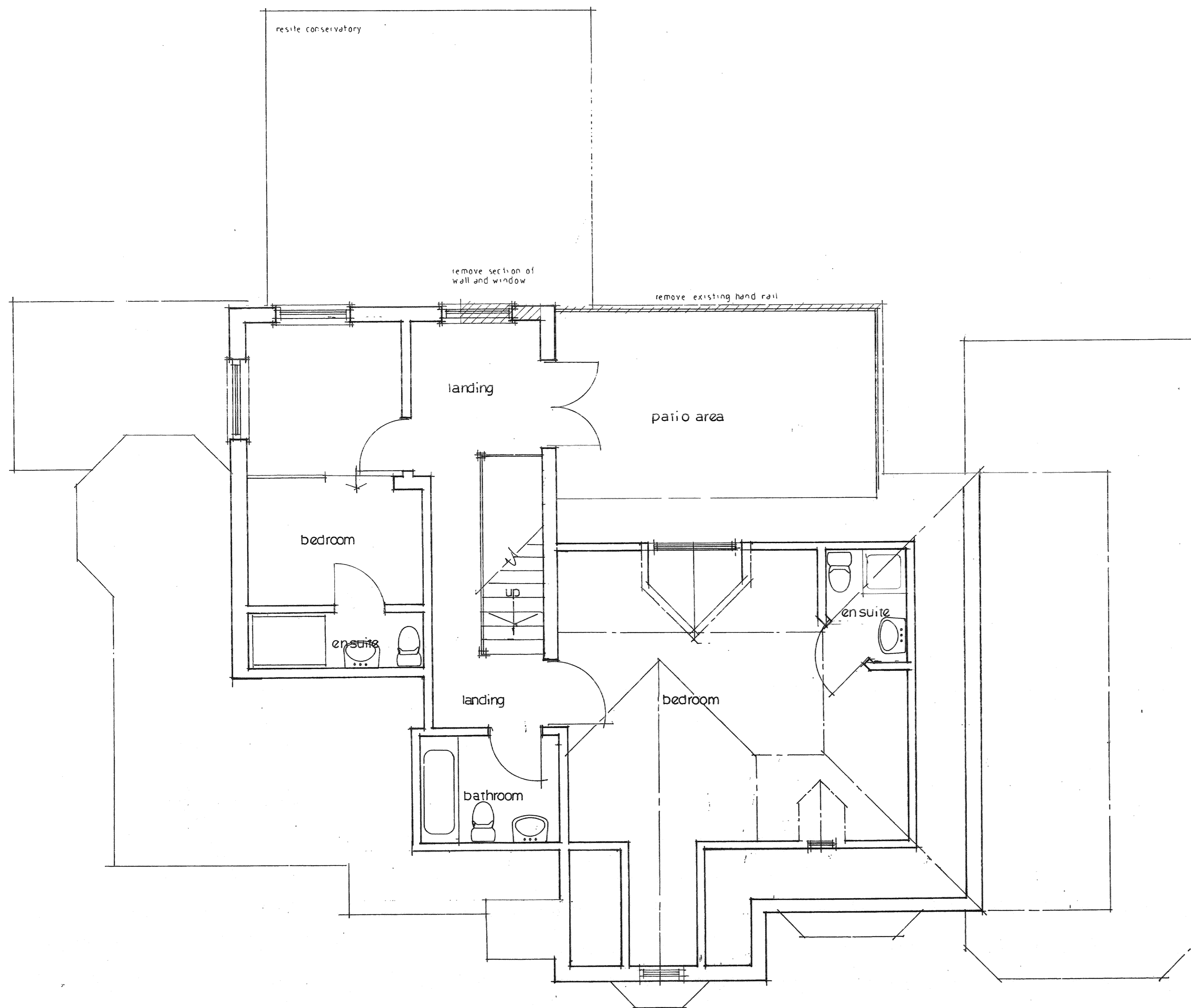
existing attic plan scale 1/50
