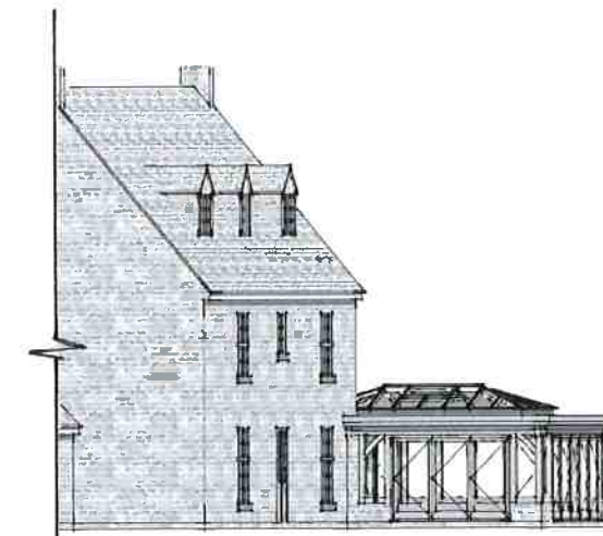
EXISTING SOUTH-WEST ELEVATION
