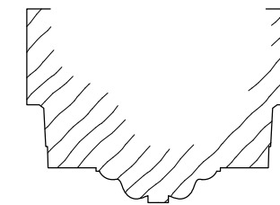
Timber Door in Bedroom 5 on First Floor IV. (Showing detail of casing between doors) (1:1)
