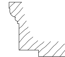
Timber Door in Bedroom 5 on First Floor V. (Showing detail of top casing) (1:1)
