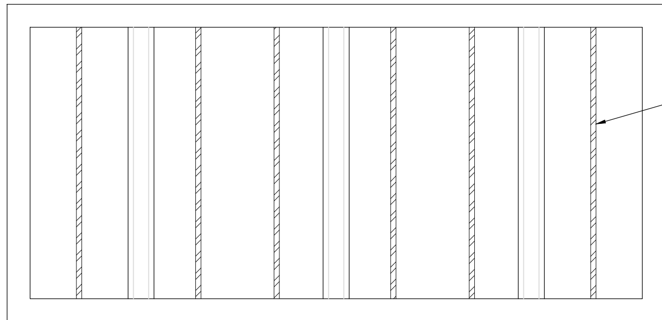
Timber Window in the Basement I. (Showing elevation to the frame) (1:10)
