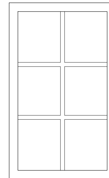
Timber Window in the Basement III. (Showing elevation to casement window) (1:10)
