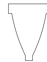
Timber Window in the Basement V. (Showing detail of glazing bar) (1:1)
