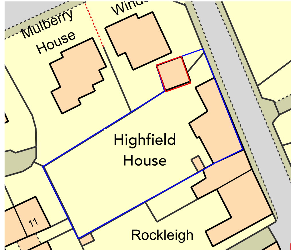
BLOCK PLAN _ AS PROPOSED Scale 1:500 @ A3
