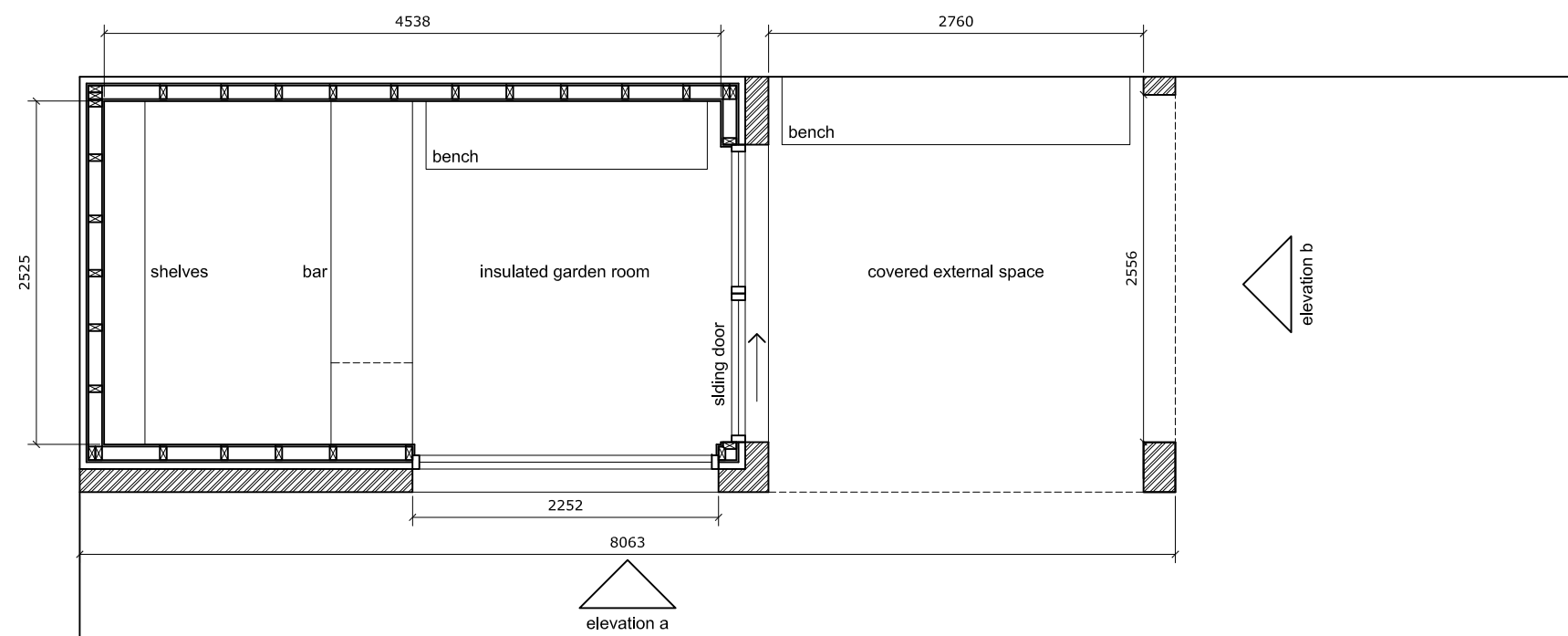
GROUND PLAN
