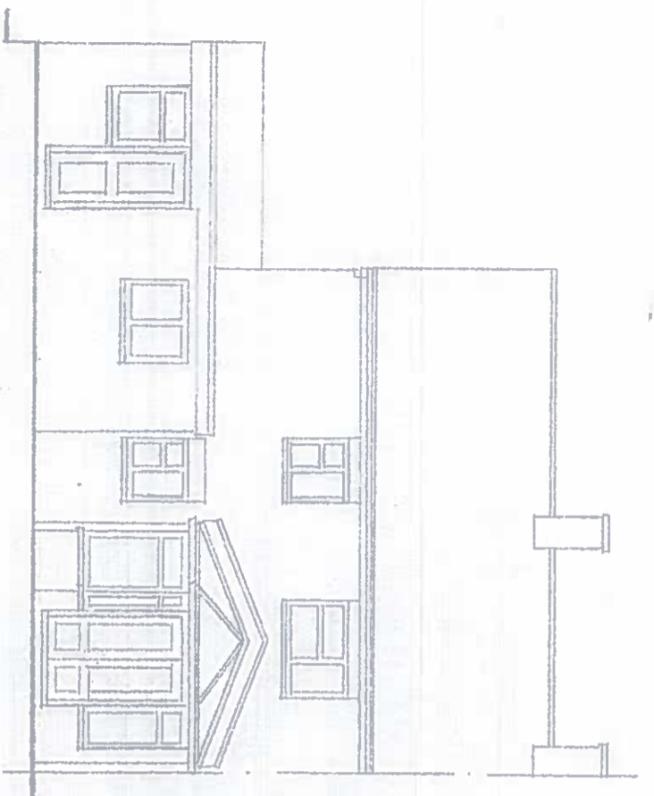
SOUTH WEST ELEVATION
