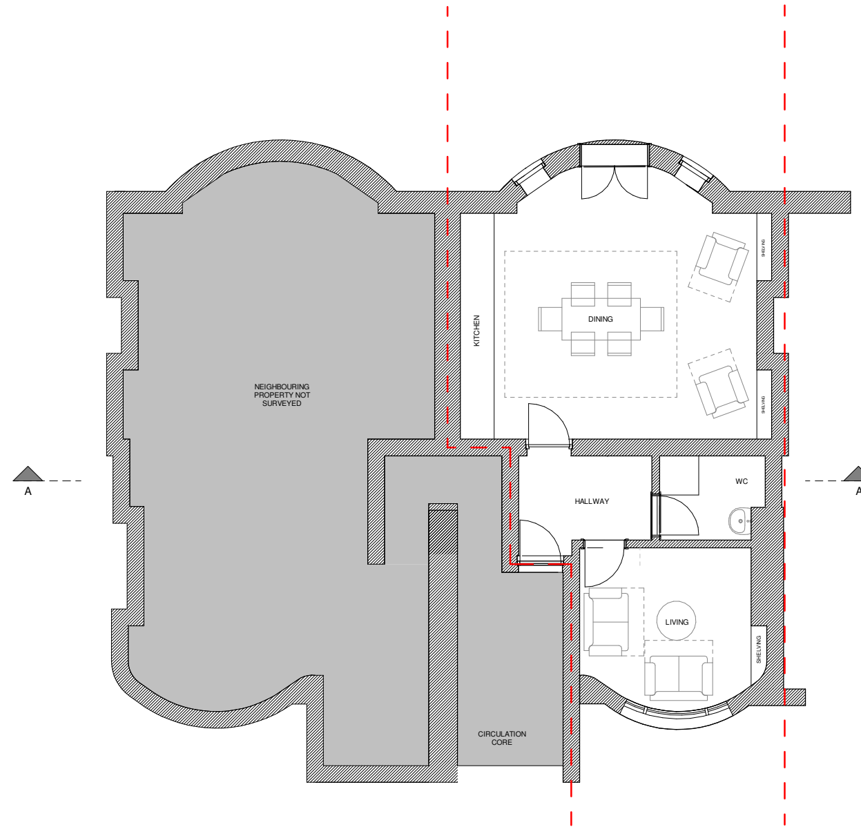
Existing Ground Floor Plan 39D 1 : 100
