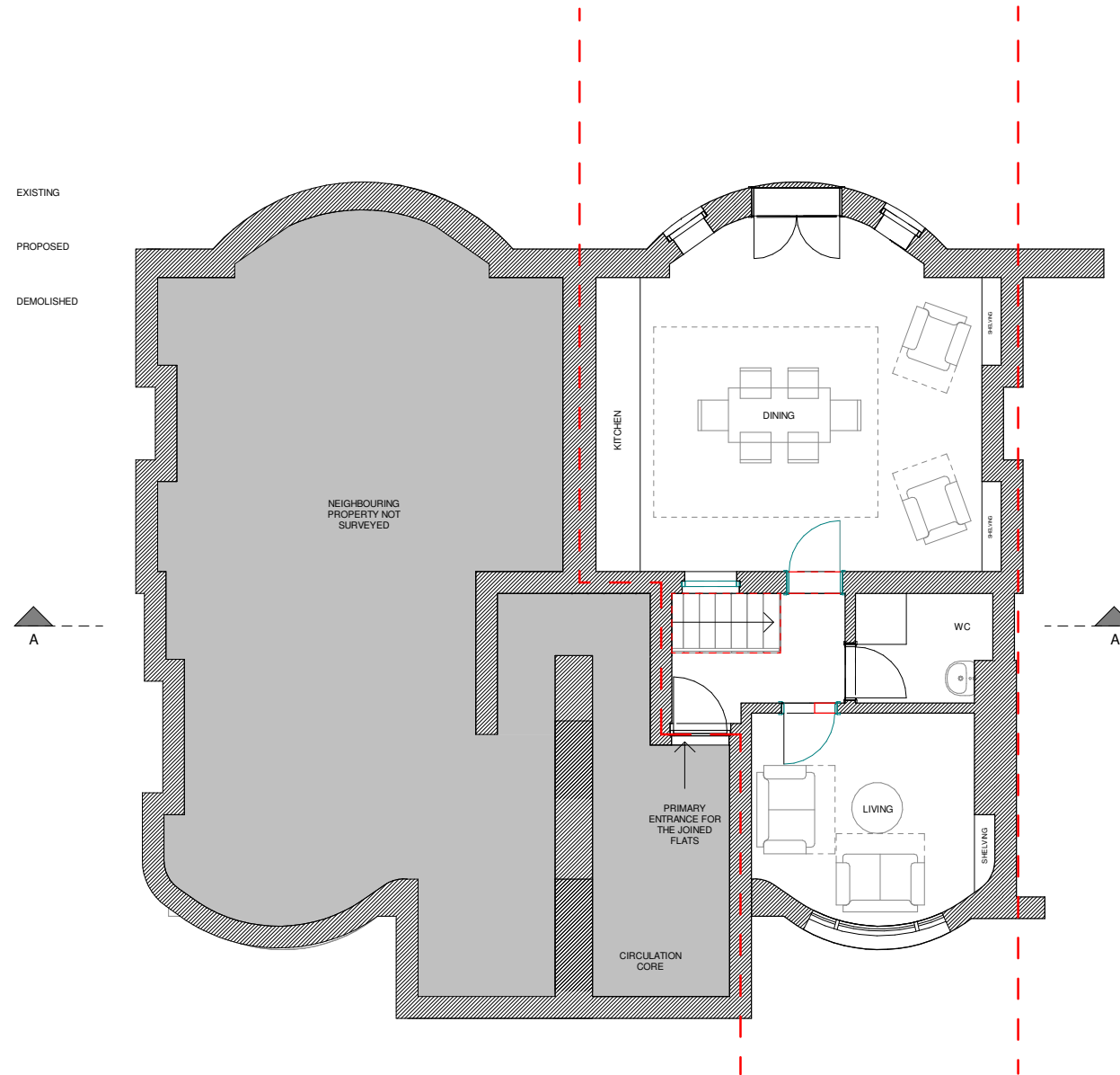
Ground Floor Plan - Revised Layout 1 : 100
