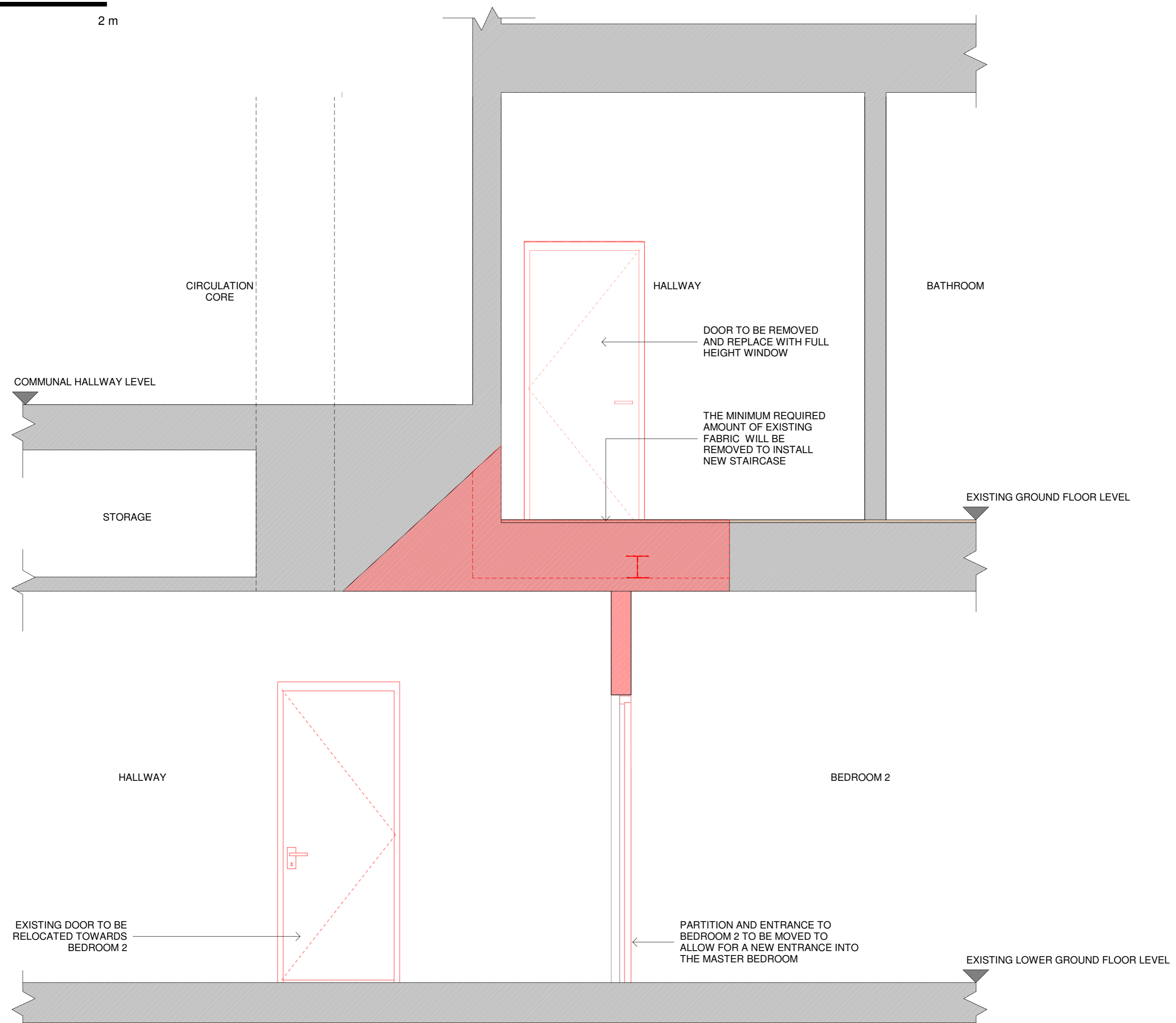
Existing & Demolition Section AA 1 : 20
