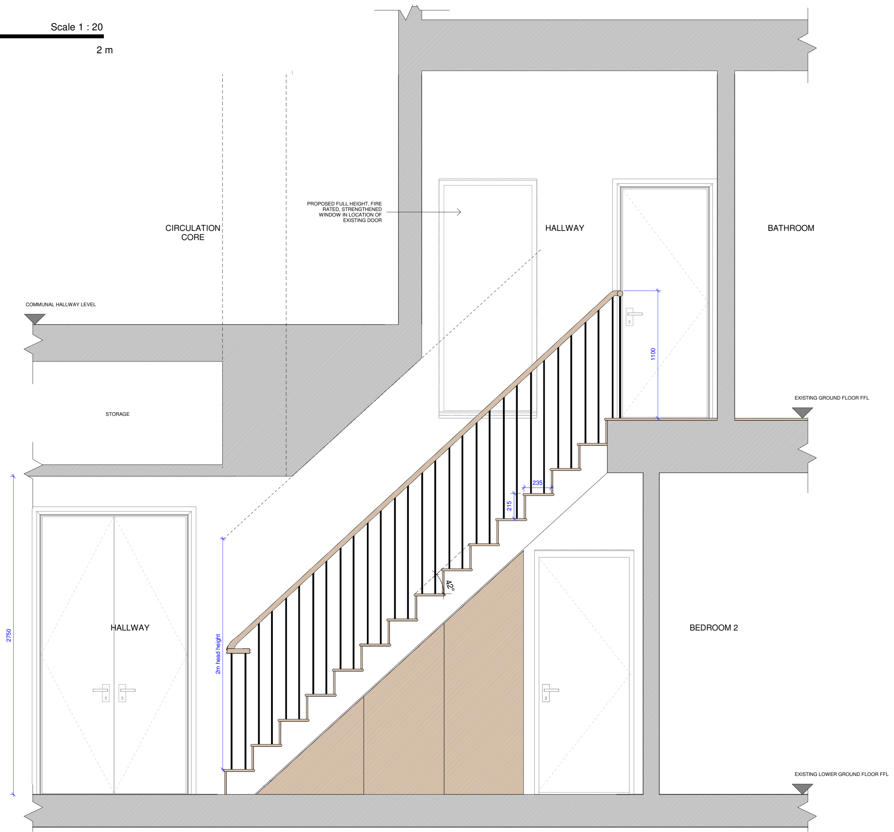
Proposed - Section AA 1 : 20
