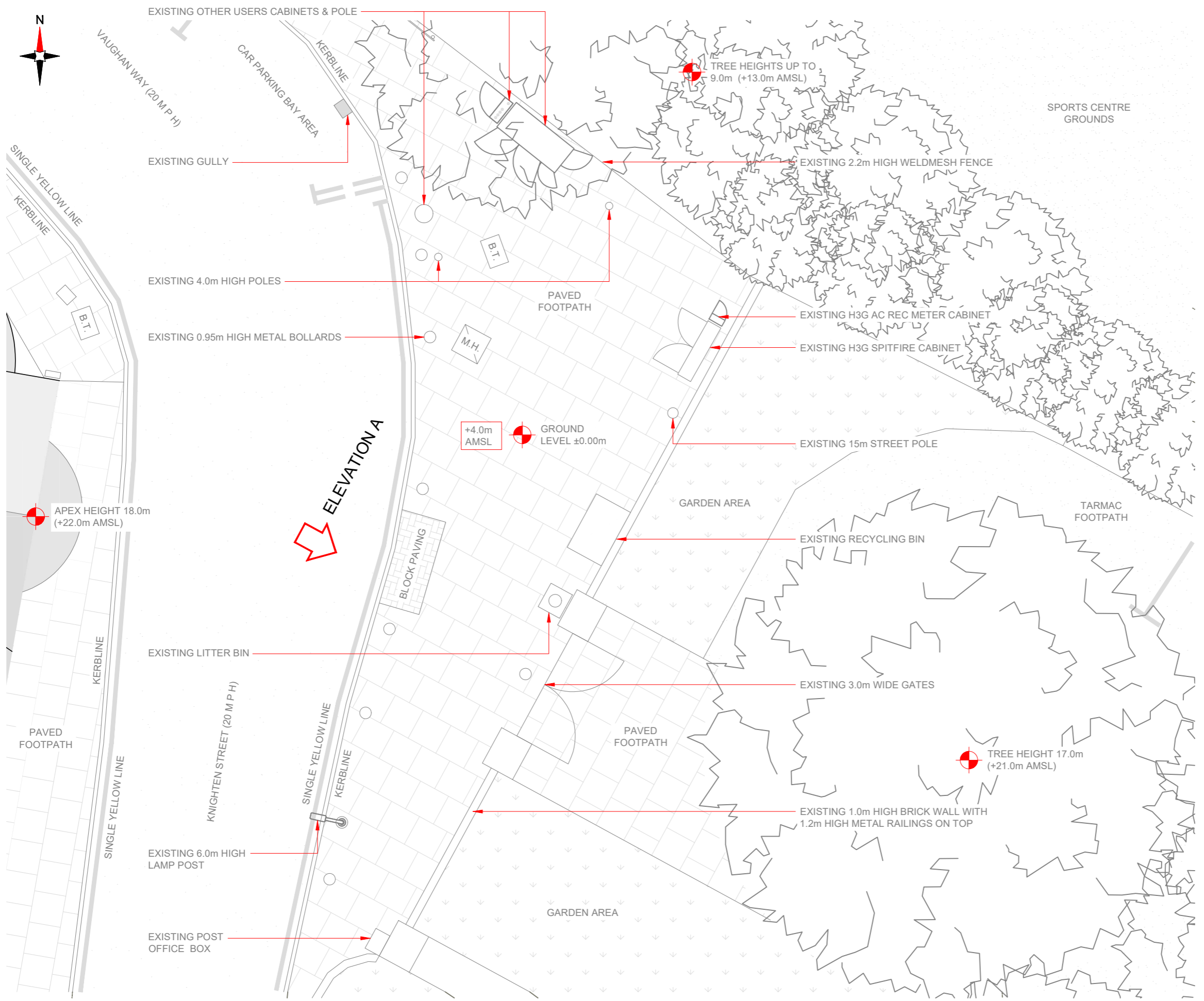
EXISTING SITE PLAN 0 1:100 2m 4
