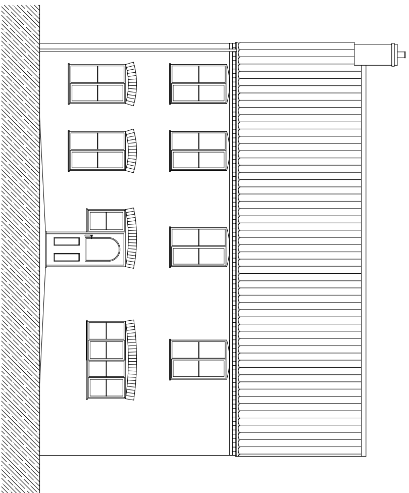
EAST ELEVATION
