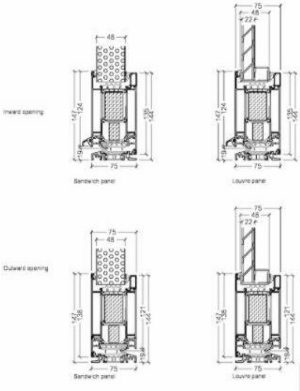
3:The sandwich panel is an aluminium door to create a special design in the door and dazzle the insight view. Up panel-value for sandwich panel: 48mm aluminium panel = 0.67 W/m²K
