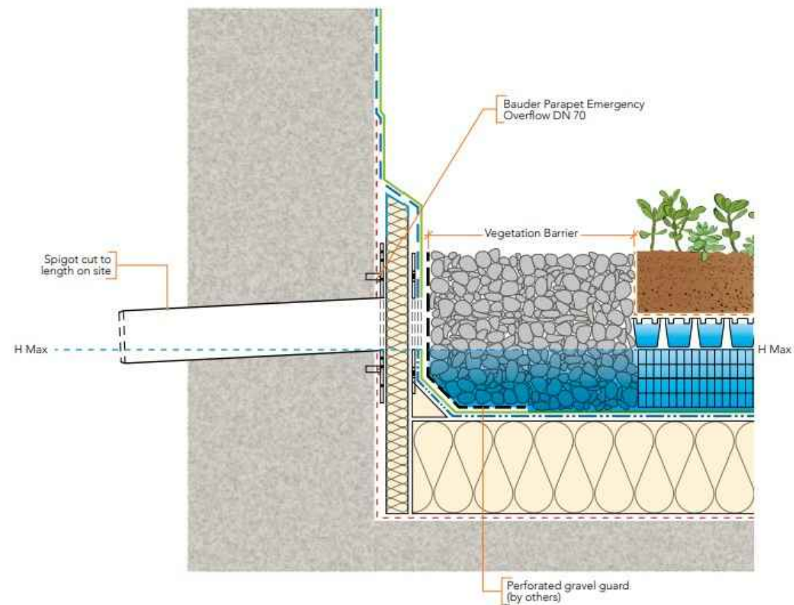
② TYPICAL BLUE ROOF BUILD-UP/OVERFLOW DETAIL (extract from the LSTA 'Rolled Lead Sheet -The complete manual')
