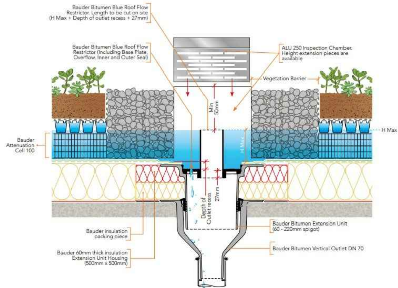
① TYPICAL BLUE ROOF BUILD-UP/OUTLET DETAIL (extract from the LSTA 'Rolled Lead Sheet -The complete manual')
