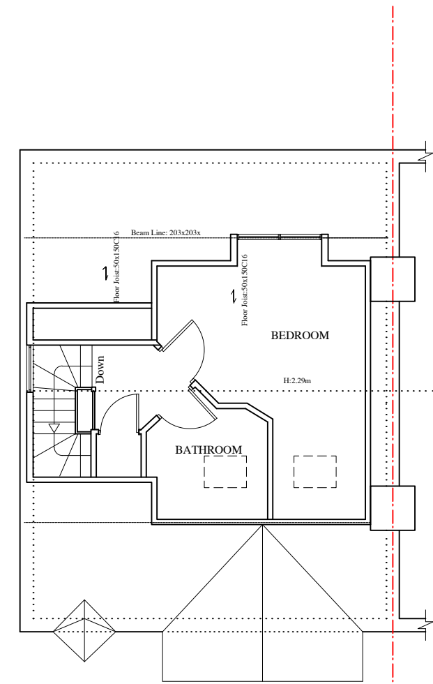
EXISTING LOFT FLOOR PLAN
