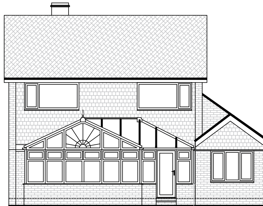
FRONT ELEVATION
