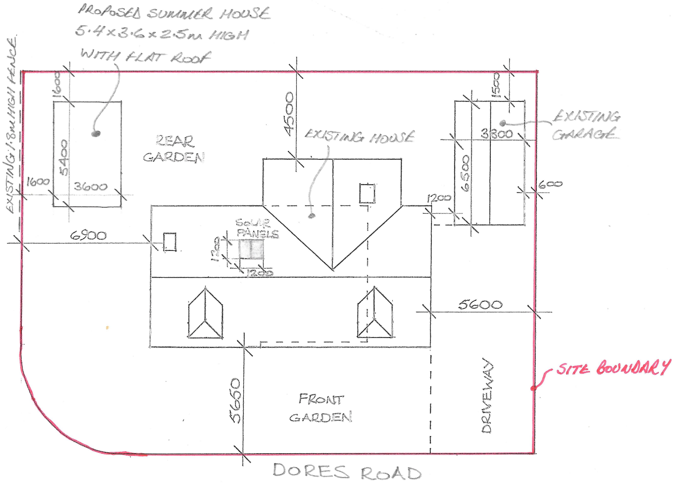
PROPOSED SITE PLAN 1:200
