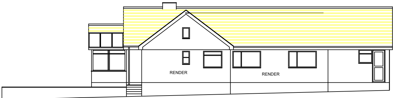
NORTH ELEVATION
