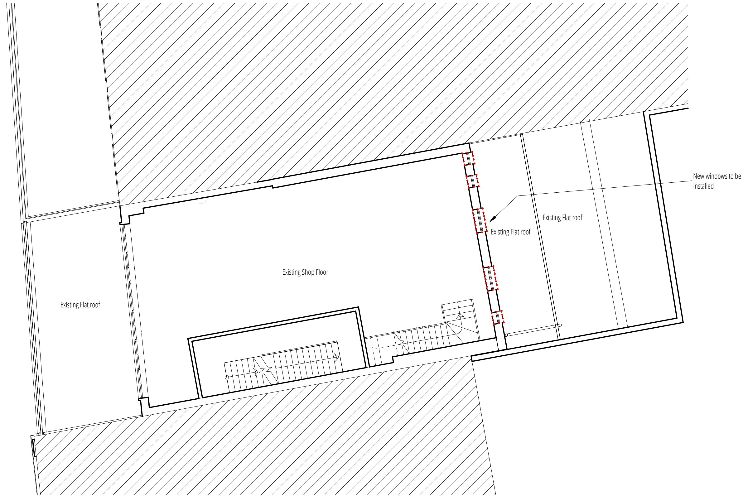
1 Proposed First floor 1 : 100
