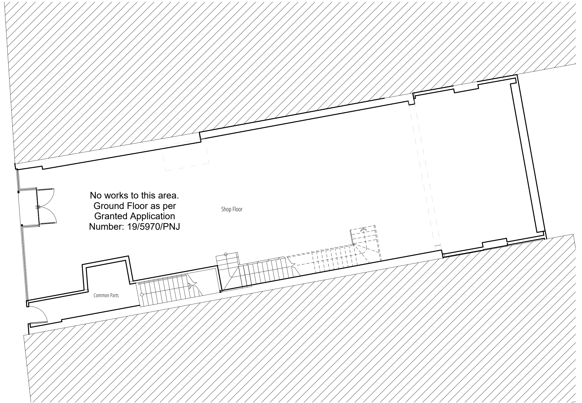
① Existing Ground Floor Plan 1 : 100
