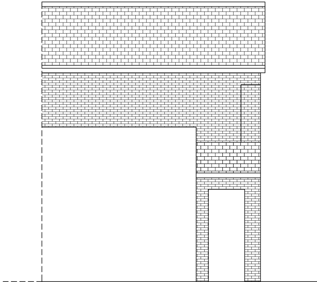
EXISTING SOUTH OUTER ELEVATION PLAN
