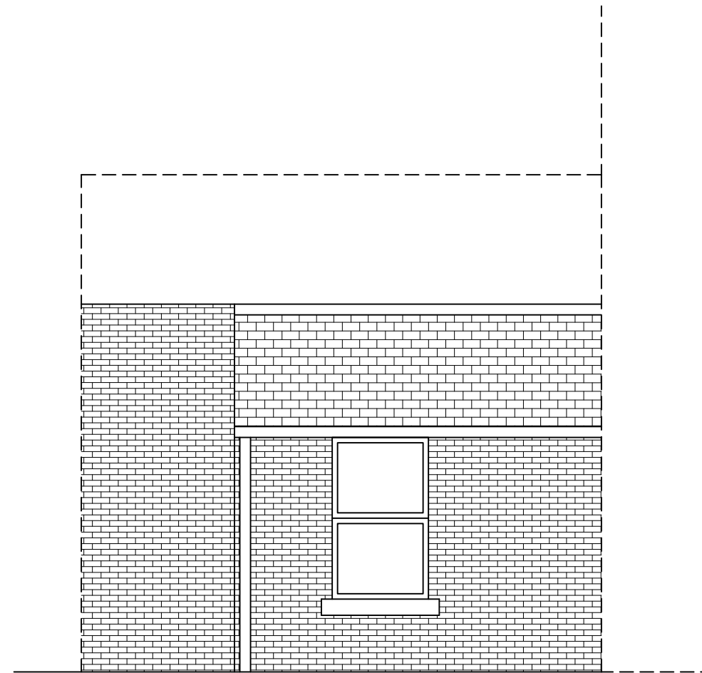
EXISTING NORTH INNER ELEVATION PLAN
