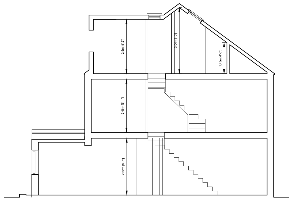
PROPOSED SECTION A
