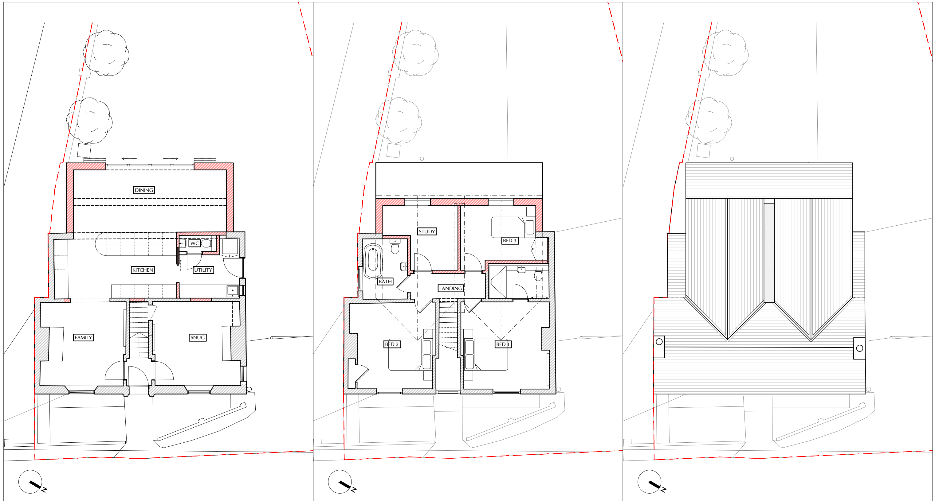
09 001 Proposed Floor Plans Ground First & Roof
