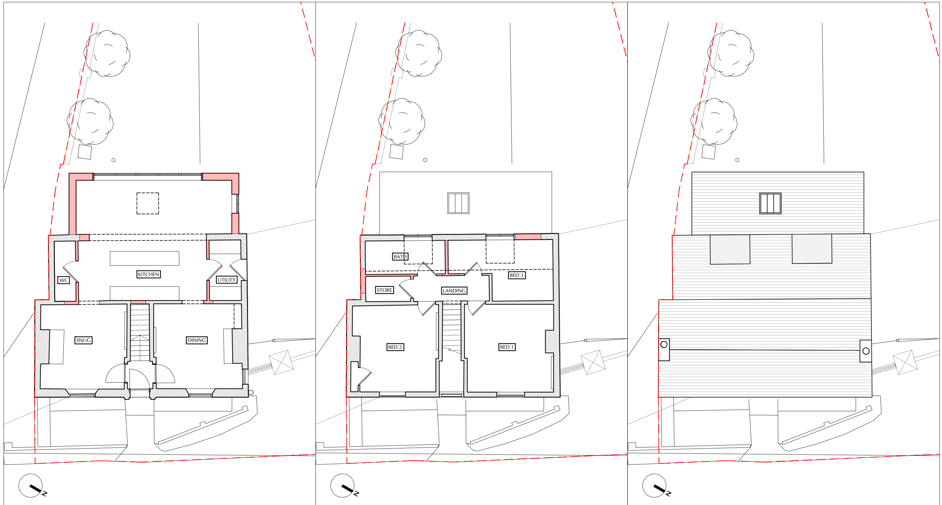
03 001 As Previously Approved Floor Plans Ground First & Roof
