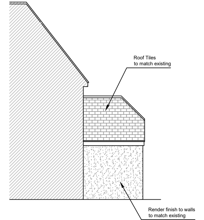
Part - Front Elevation on Utility
