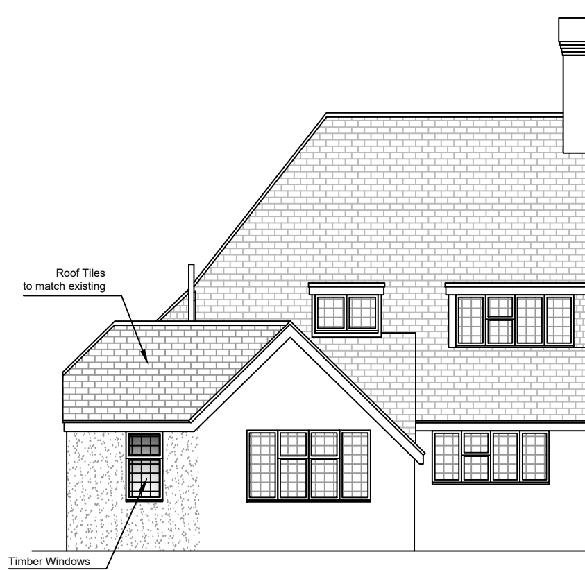
Rear Elevation
