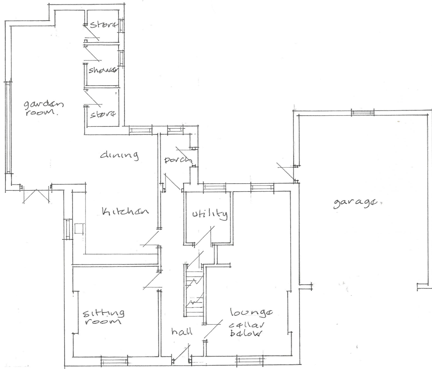
GROUND FLOOR 1:100
