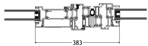
Detail B
