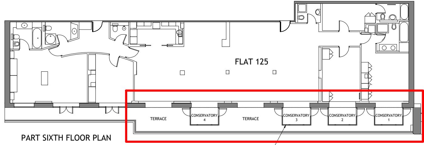
EXISTING CONSERVATORIES FOUR INDEPENDANT UNITS
