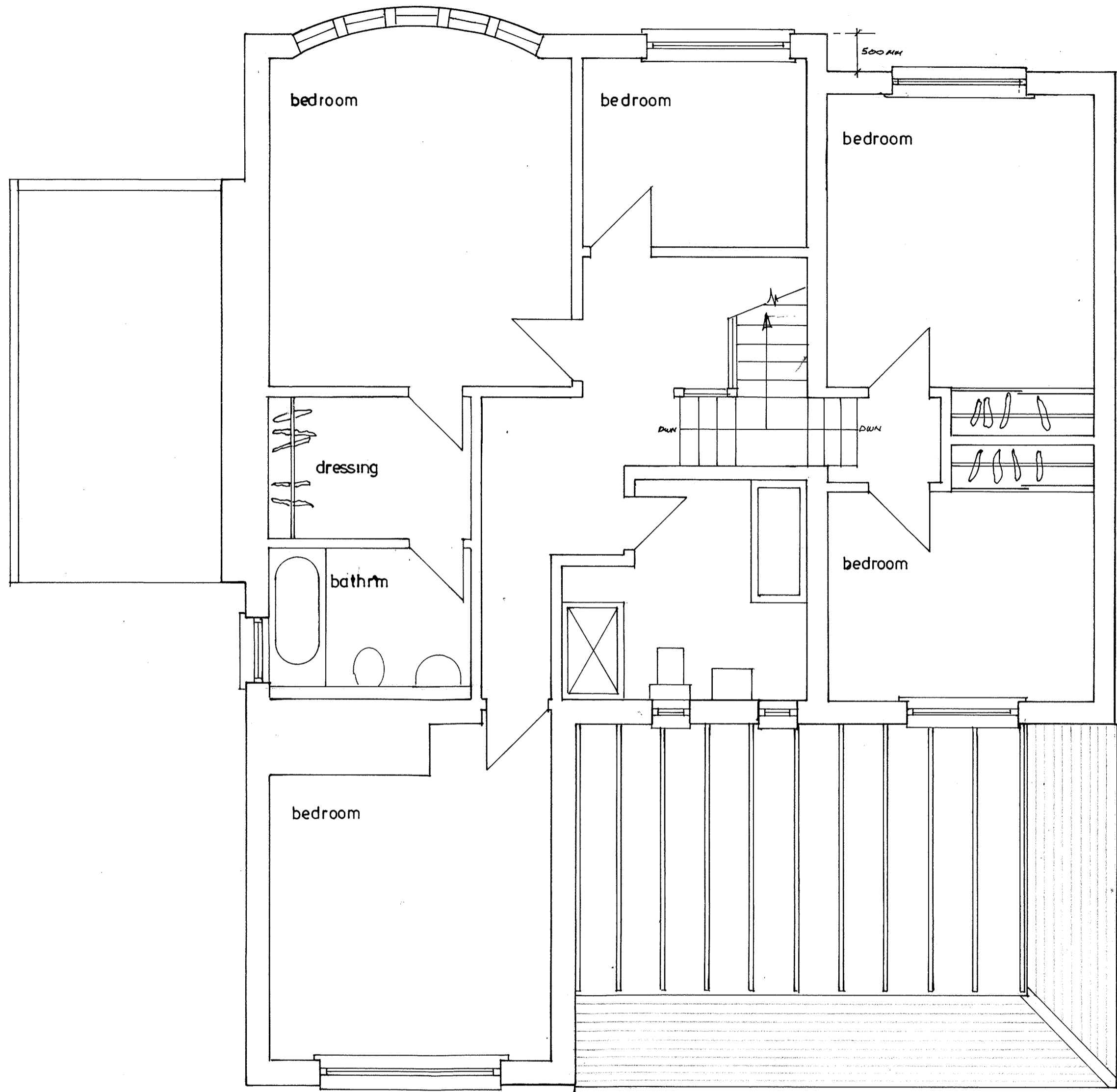
UPPER FLOOR PLAN AS PROPOSED
