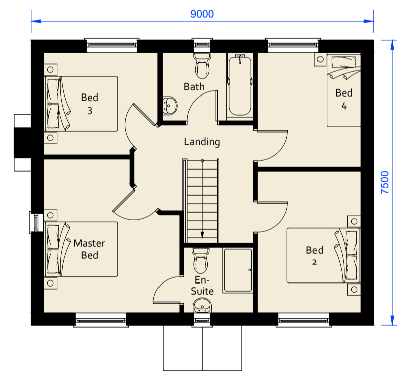
Proposed 1st Floor Plan
