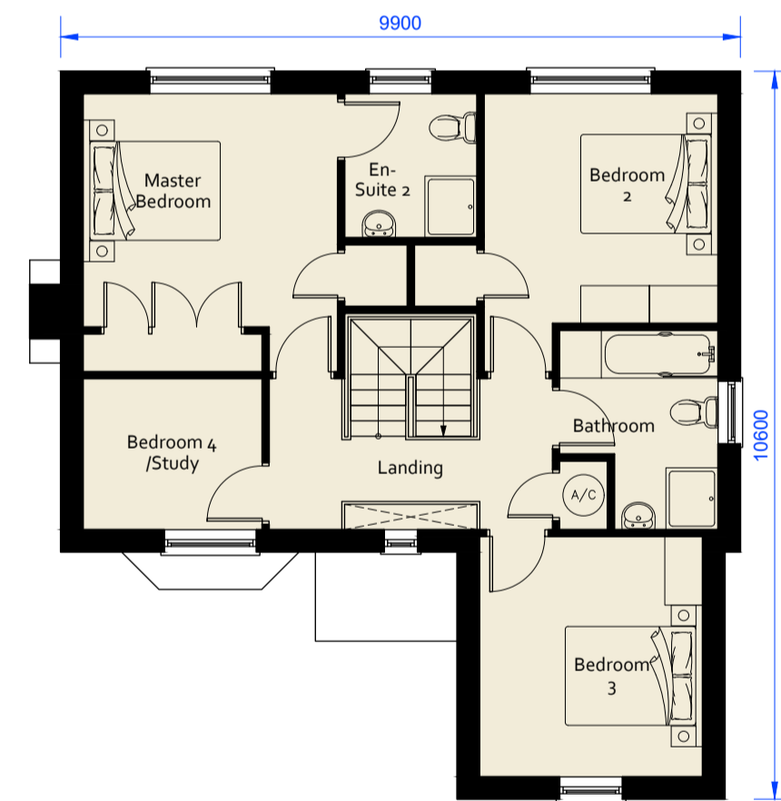
Proposed 1st Floor Plan
