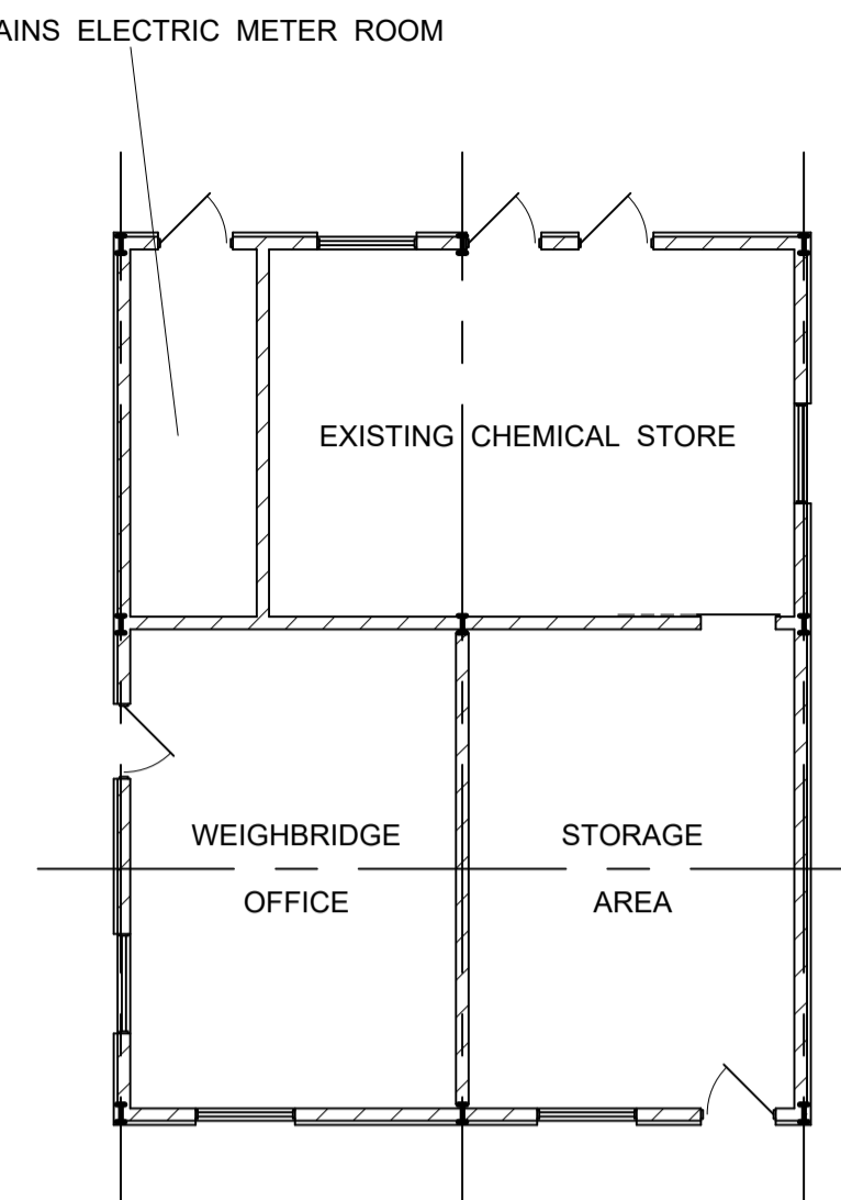
FLOOR PLAN
