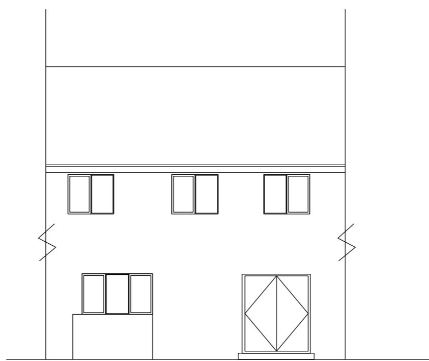
REAR ELEVATION
