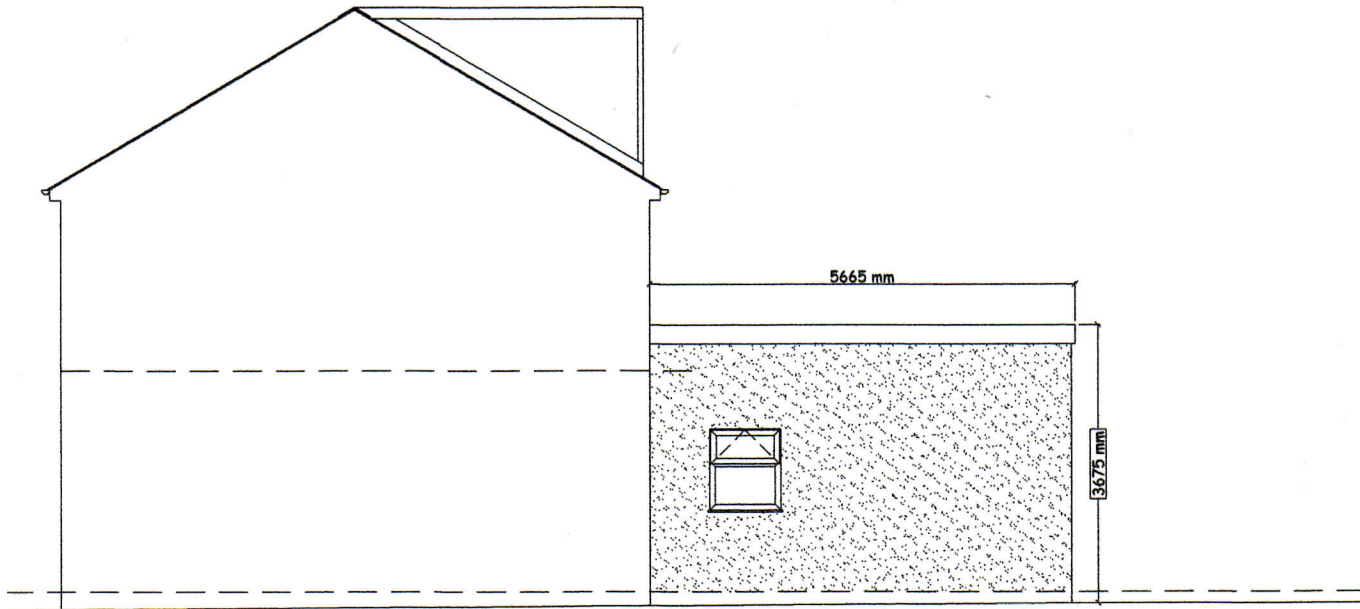
Side 2 elevation
