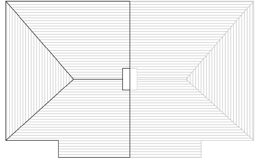
ROOF PLAN
