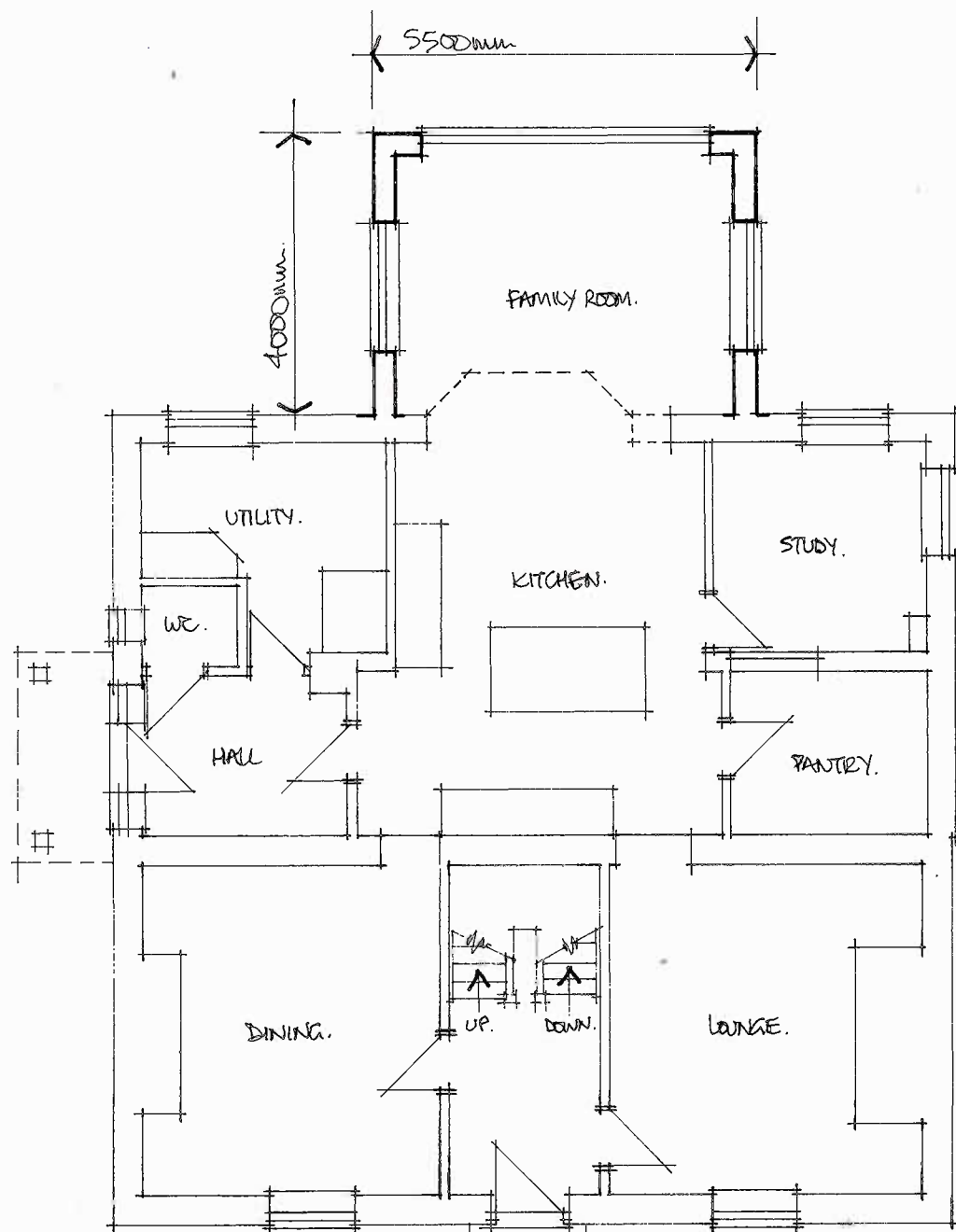
ground floor. 1:100.
