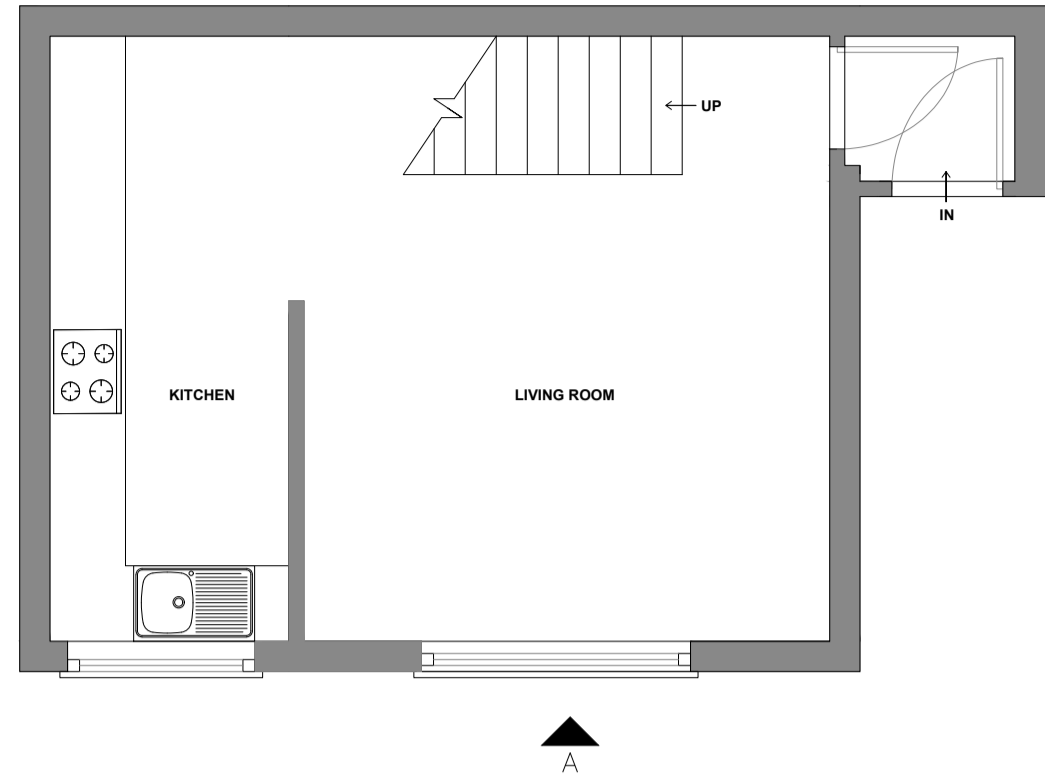
01 EXISTING FLOOR PLAN Scale: 1:50 @ A1
