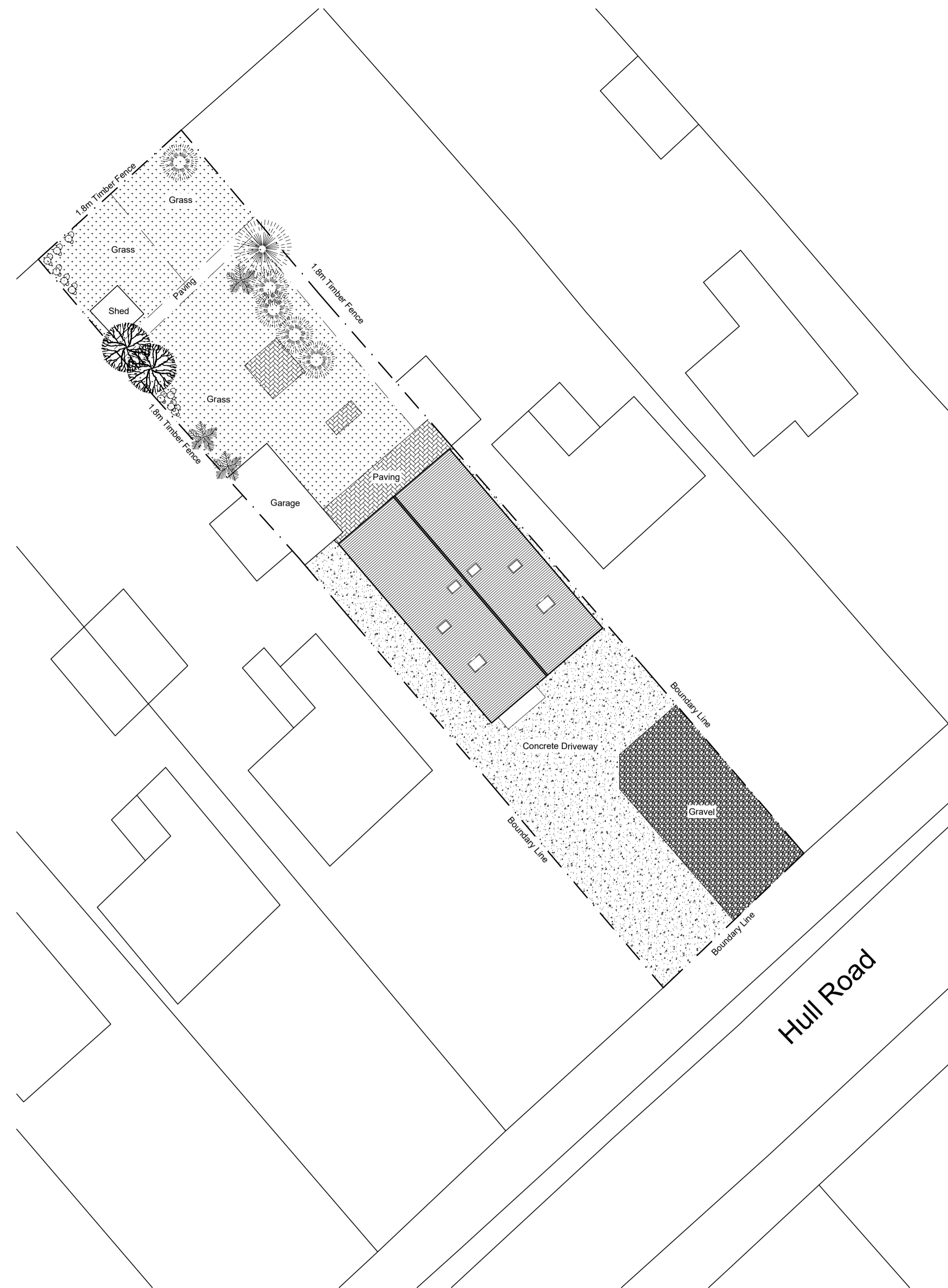
Proposed Block Plan @ 1:200 A1
