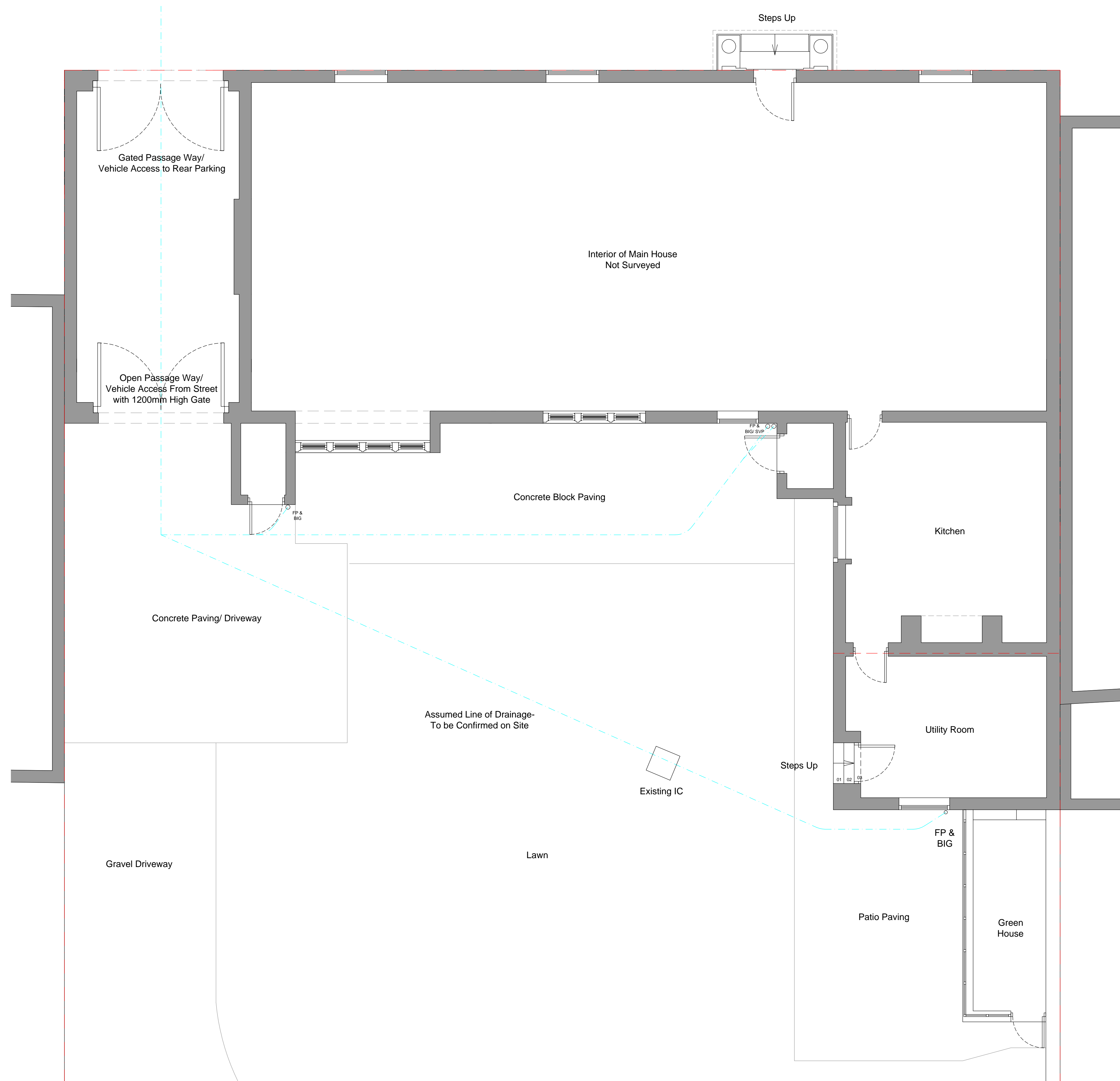
Existing Ground Floor Plan 1:50
