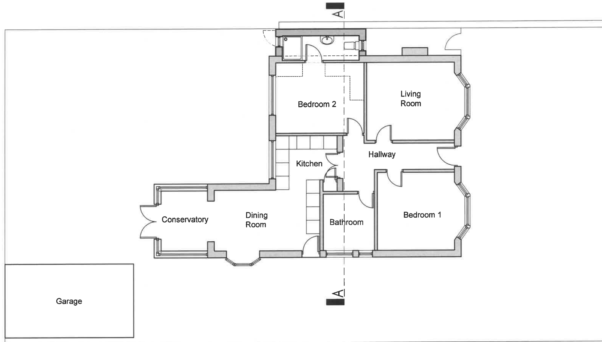
Ground Floor
