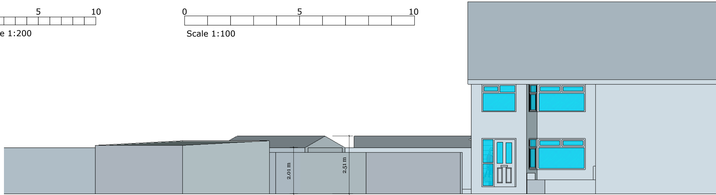
Front (South) Elevation
