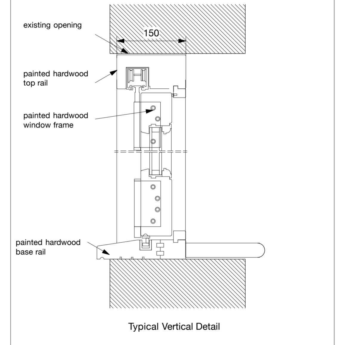
Detail Through Proposed Shopfront scale 1:5
