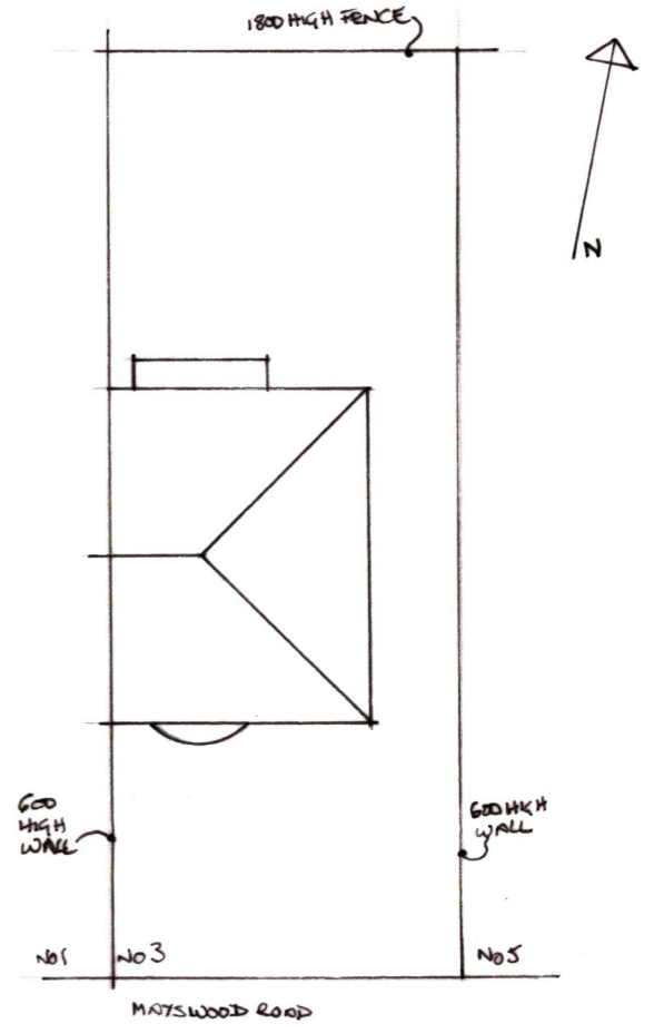
EXISTING SITE AND ROOF PLAN 1:200
