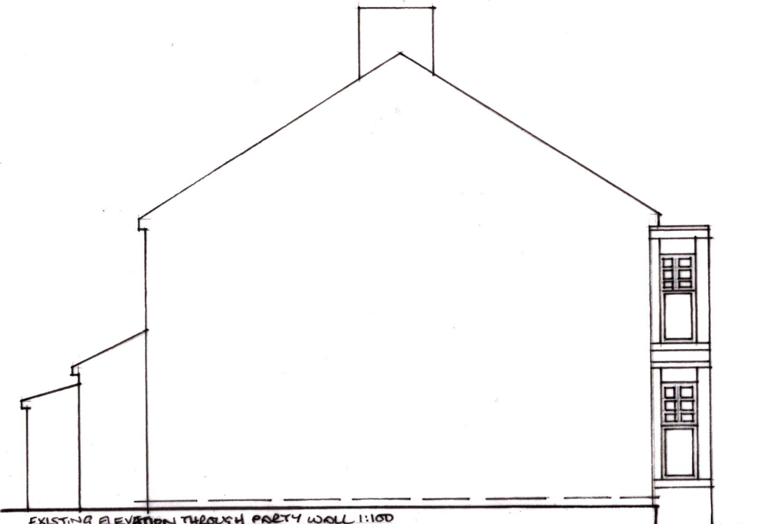
EXISTING ELEVATION THROUGH PARTY WALL 1:100
