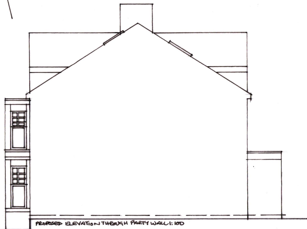
PROPOSED ELEVATION THROUGH PARTY WALL 1:100
